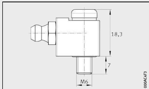
Lubrication connector S62 3)
