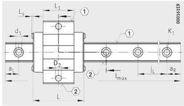
KUV...-B-EC View X rotated 90°
