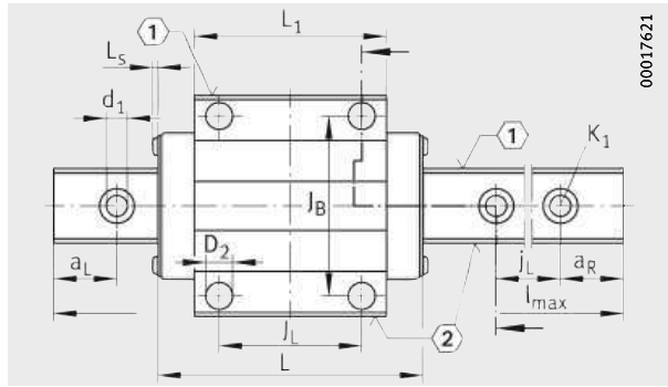
KUVE...-B-E View X rotated 90°
