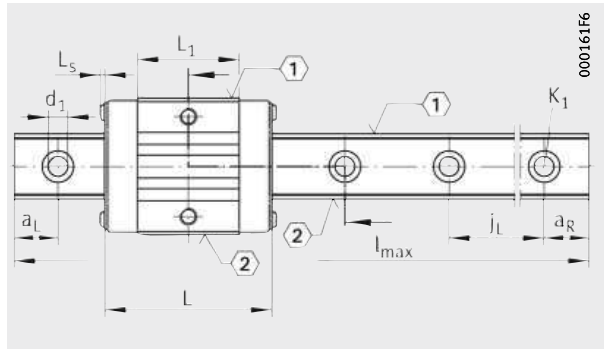
KUVE..-B-ESC View X rotated 90°
