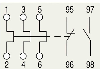
Overload Relay
